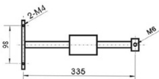
Horizontal Install
